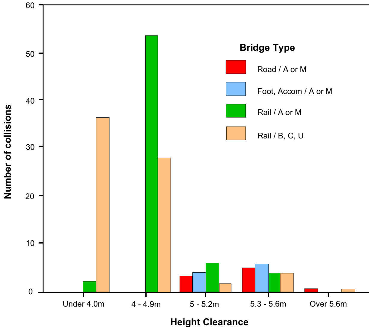
FIG A/1 DISTRIBUTION OF BRIDGE DECK COLLISIONS (England and Wales 1989 - 1990)
