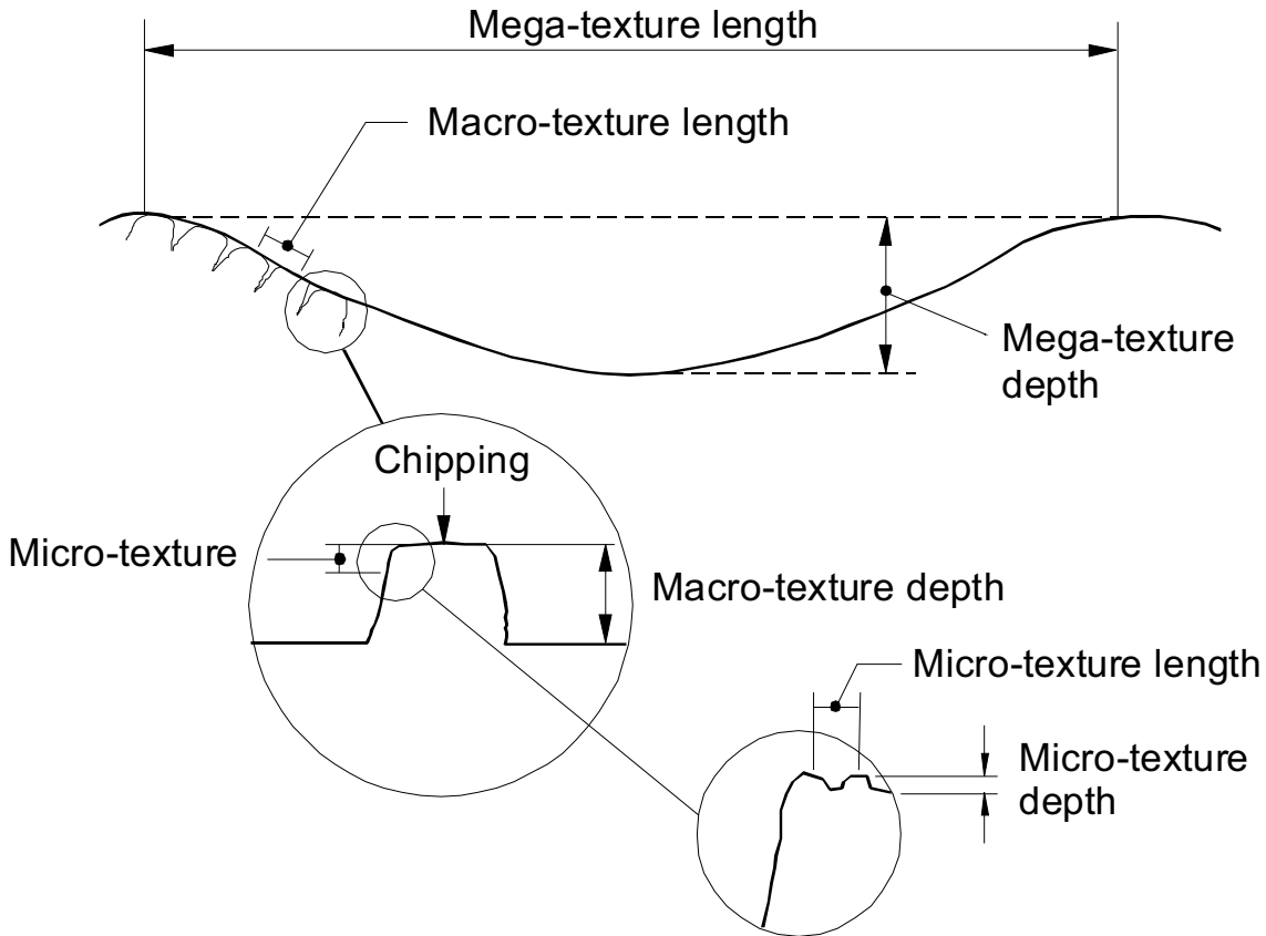
Figure 5.1 Details of texture length and depths
