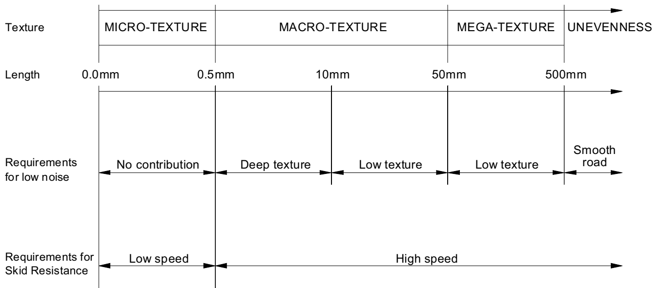
Figure 5.2 Effects of texture depths on skidding and noise
