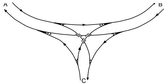
(b) Major Merge/Diverge Layout with Direct Links
