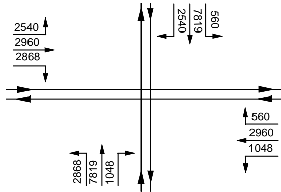
(a) Traffic Flow Diagram
