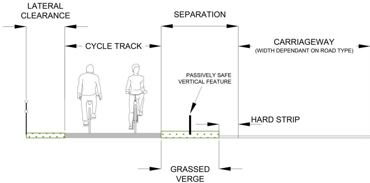
Figure 3.3: Off-Road Two-Way Cycle Track
