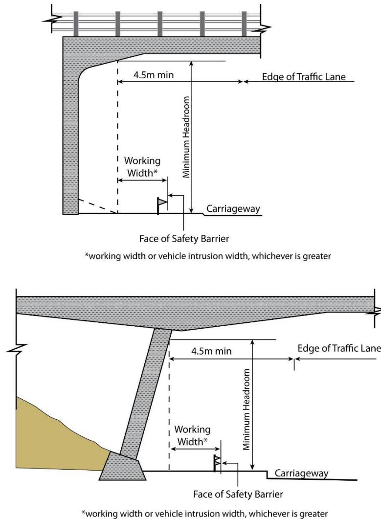
Figure 5.1: Headroom at Structures
