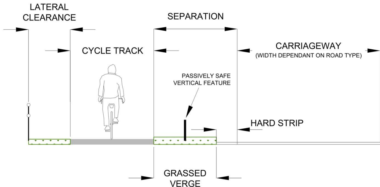
Figure 3.2: Off-Road One-Way Cycle Track
