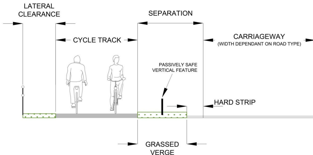
Figure 3.3: Off-Road Two-Way Cycle Track
