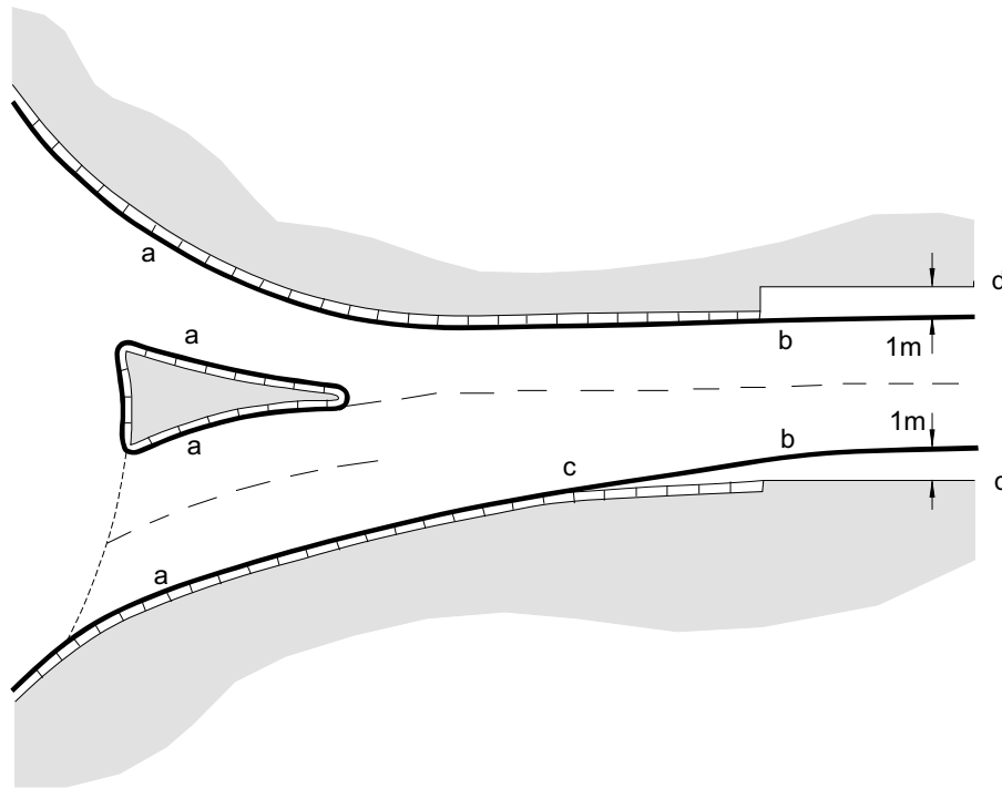
Method of Terminating Edge Strips on Single Carriageway Approach to a Roundabout Figure 7/9
