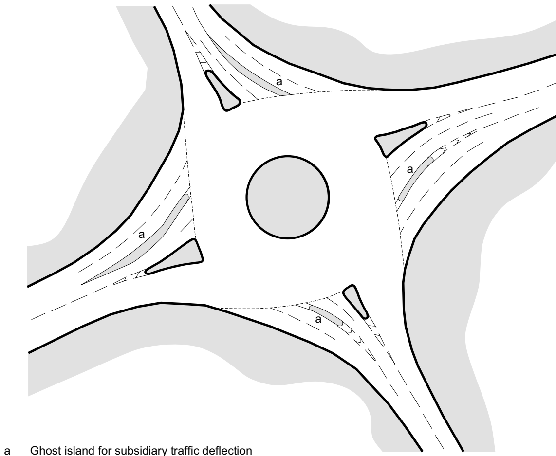
Entry Deflection Achieved by Subsidiary Traffic Deflection Islands
