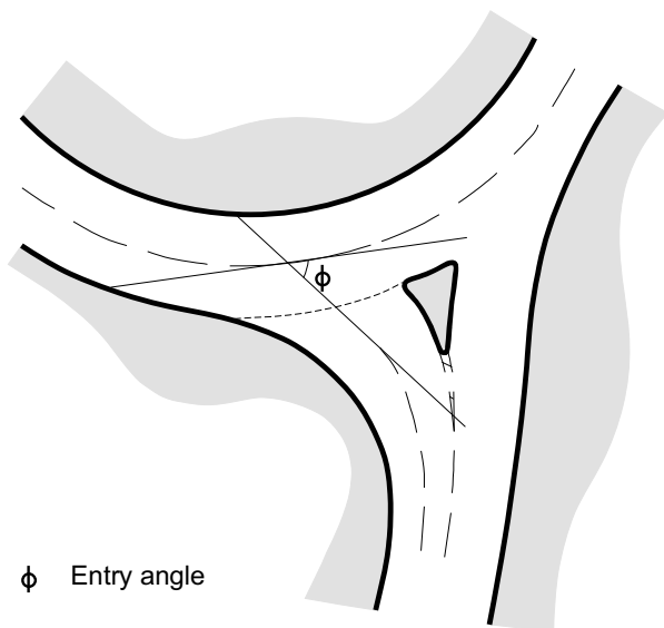
Example of Too High an Entry Angle and also Excessive Entry Deflection
