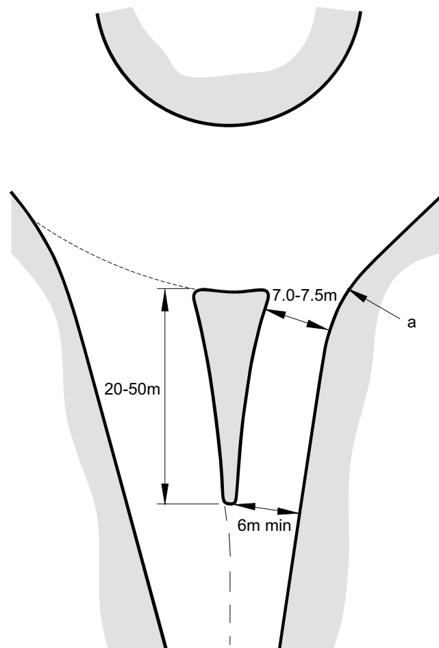
a Exit radius 40-100m
