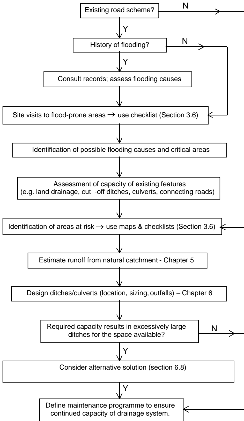
Figure 1 – Methodology Flowchart
