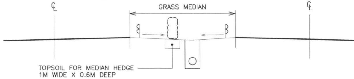
NORMAL CARRIAGEWAY WITH FILTER DRAIN
