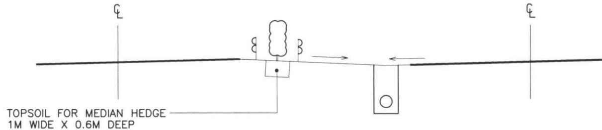
LEFT HAND CURVE WITH RIGHT HAND SIDE FILTER DRAIN OR CARRIER DRAIN
