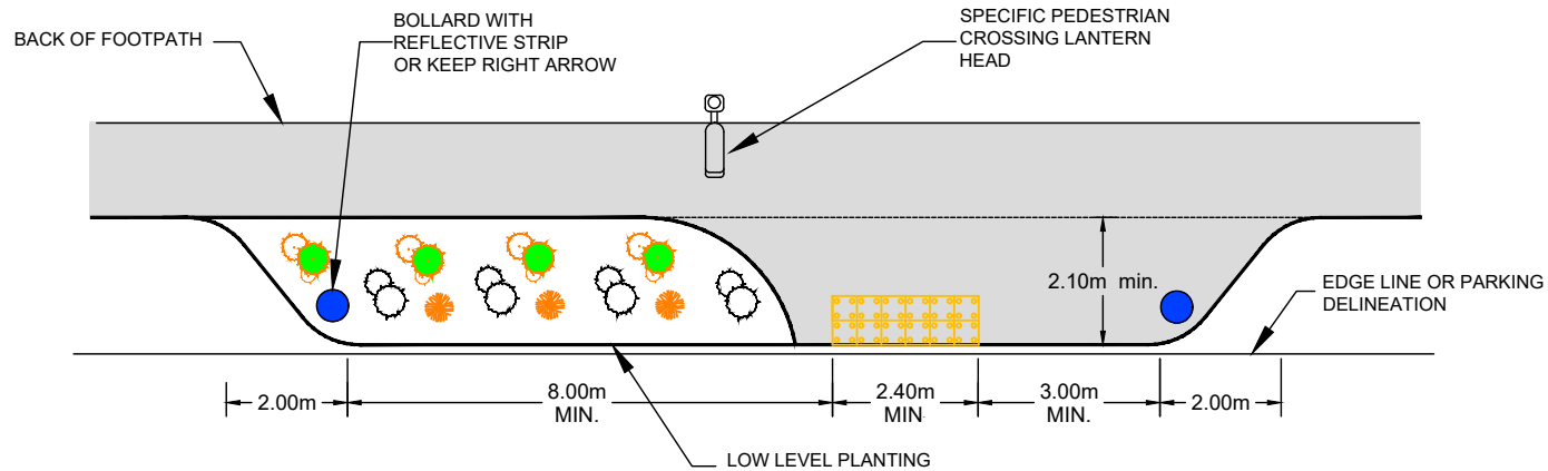
B: WITH PEDESTRAIN FACILITY
