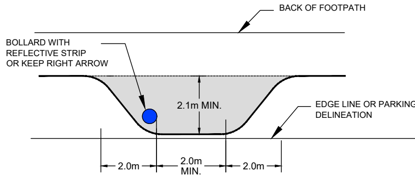
A: WITHOUT PEDESTRAIN FACILITY
