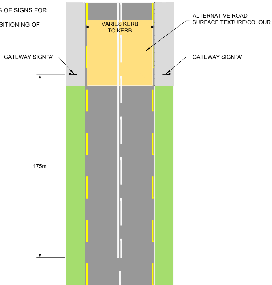
PLAN OF ROAD ON APPROACH TO GATEWAY TYPE A DESIGN
