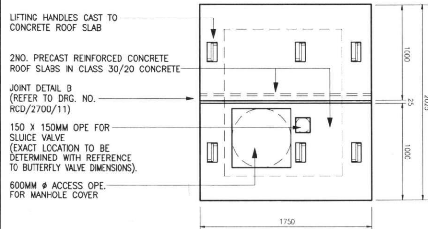
ROOF PLAN
