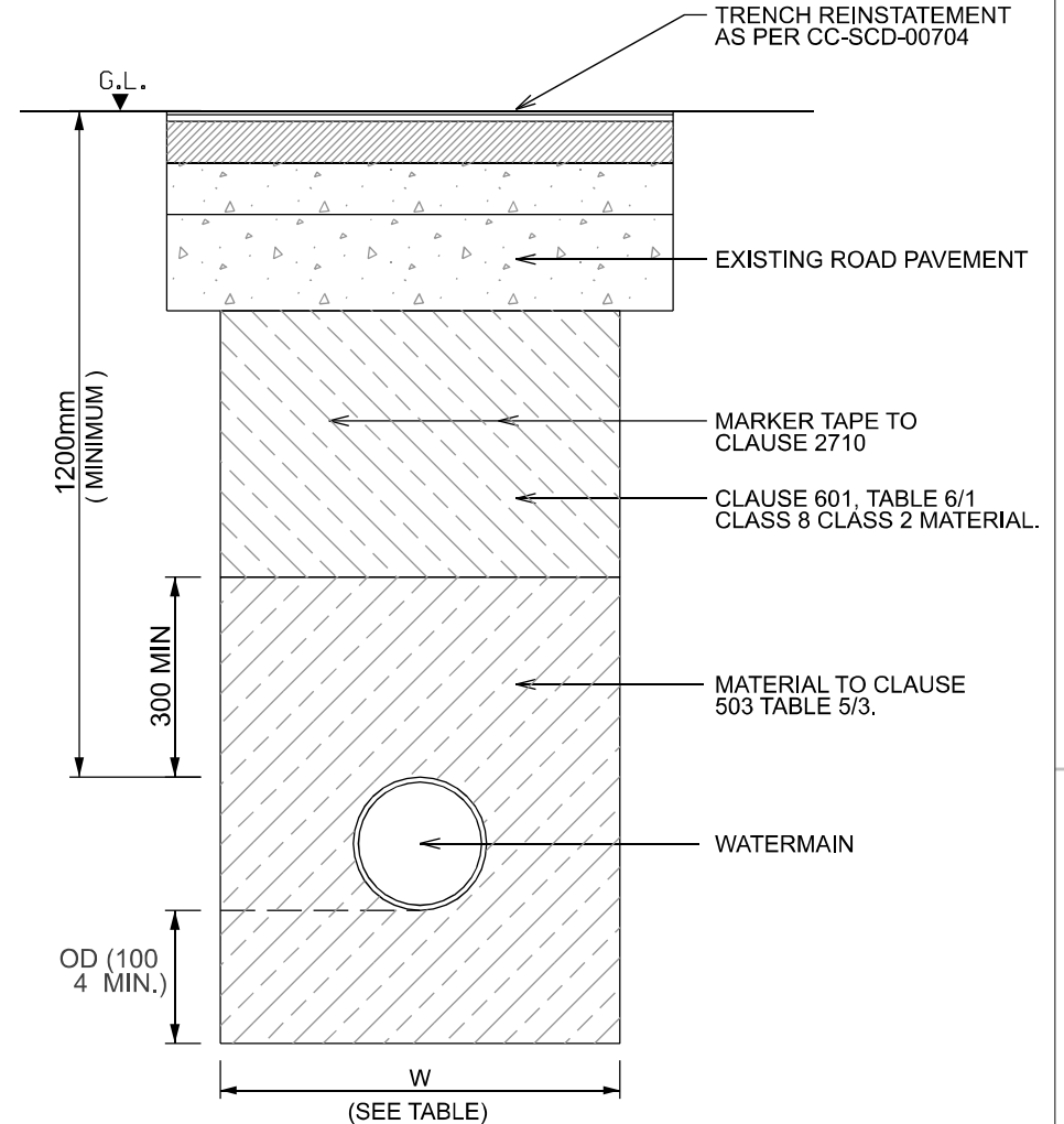
TRENCH DETAIL WHERE MINIMUM COVER PROVIDED
