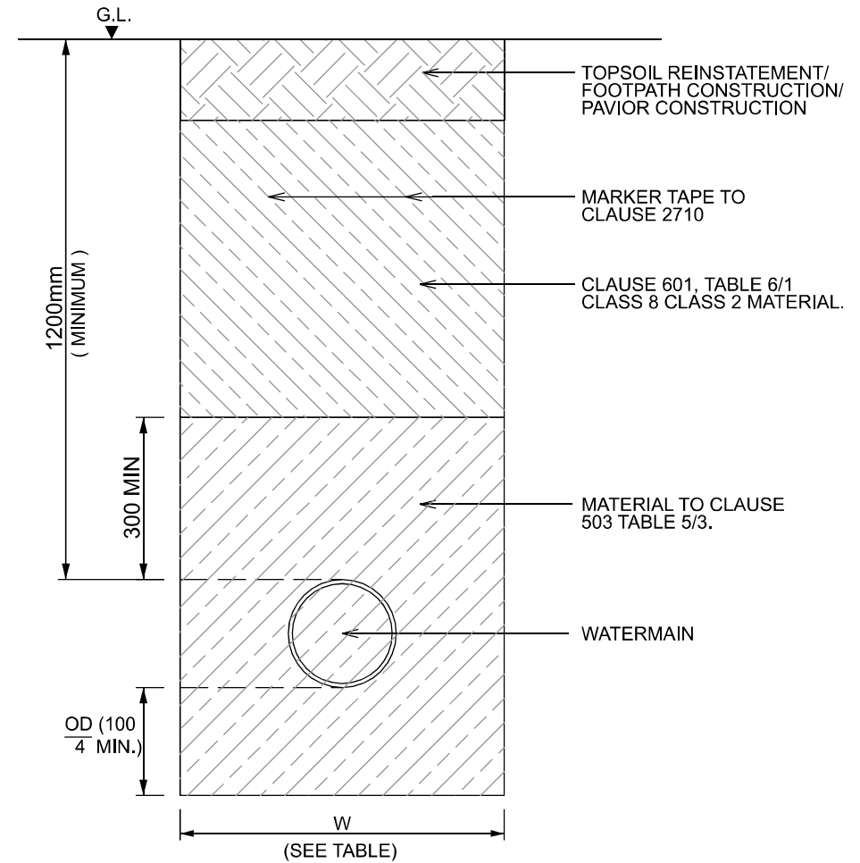
TRENCH DETAIL WHERE MINIMUM COVER PROVIDED
