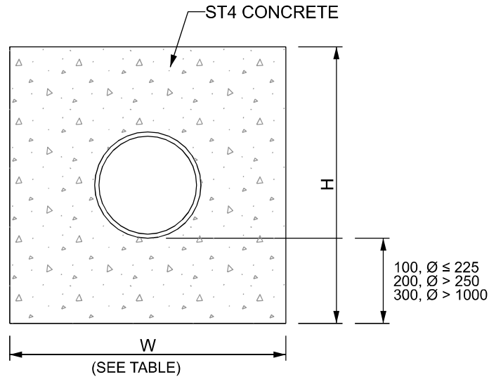
TRENCH DETAIL WHERE MINIMUM COVER NOT PROVIDED
