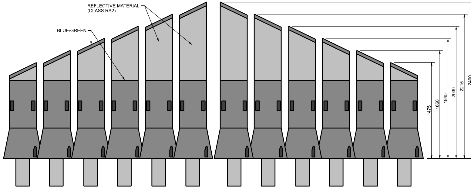
NOSING MARKER ROAD POLE
