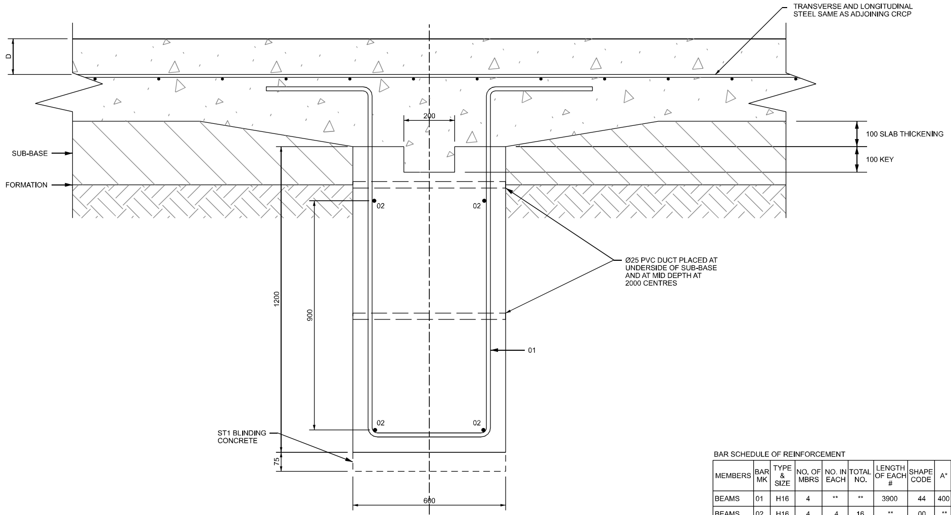
GROUND BEAM (4 NO. IN ANCHORAGE)
