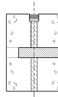
3. JOINT SEALED
