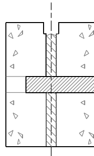
2. JOINT AFTER SAWING
