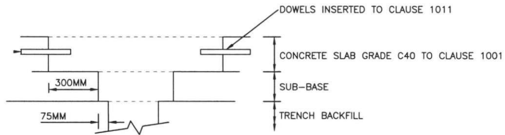
UNREINFORCED CONCRETE SLAB
