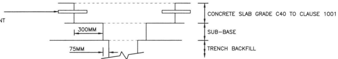
JOINTED REINFORCED CONCRETE SLAB
