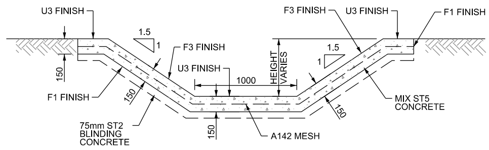
CONCRETE LINED DITCHES - D1
