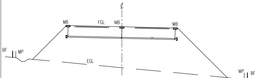
DUCT CROSSING TYPE 2 (FILL AREAS)
