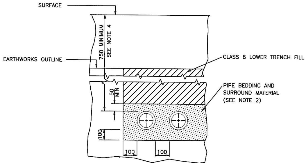
TYPE C NON-TRAFFICKED DUCTS (MINIMUM 750 COVER)
