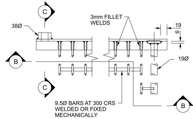
PART ELEVATION
