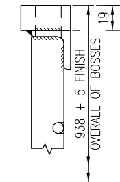
VIEW C-C
