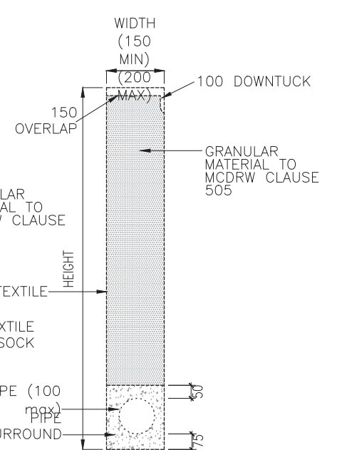
DRAIN TYPE 9 LINED TRENCH
