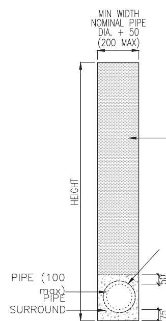
DRAIN TYPE 8 WRAPPED PIPE
