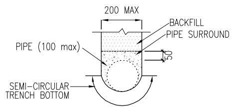
ALTERNATIVE TRENCH SHAPE FOR DRAIN TYPES 6, 7, 8 AND 9
