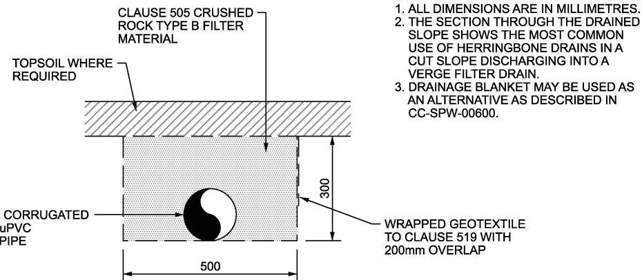
SECTION A-A SECTION THROUGH HERRINGBONE DRAINS
