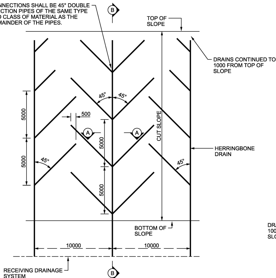
PLAN LAYOUT OF HERRINGBONE DRAINS
