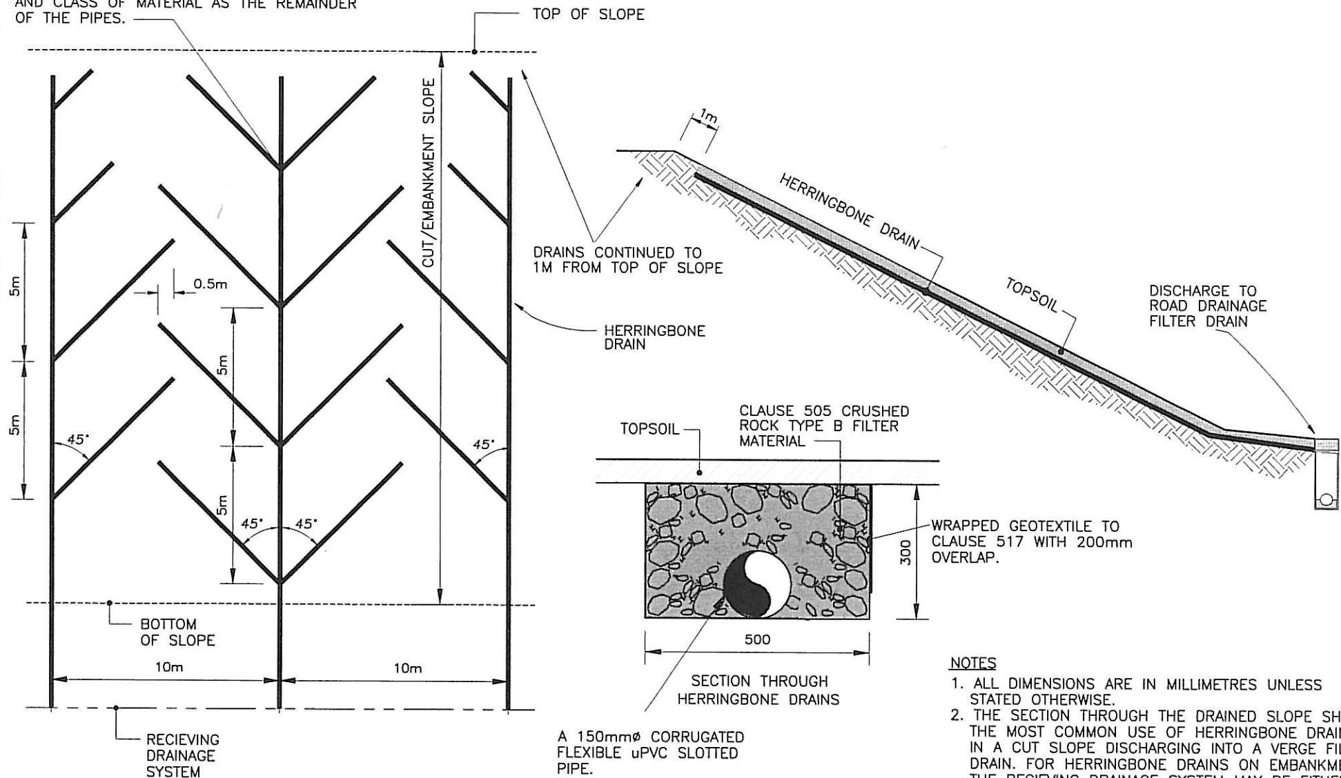
LAYOUT OF HERRINGBONE DRAINS
