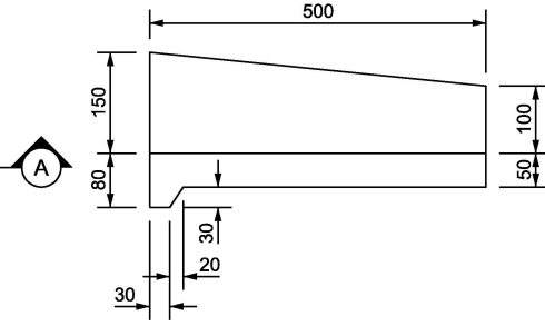
SECTION A
