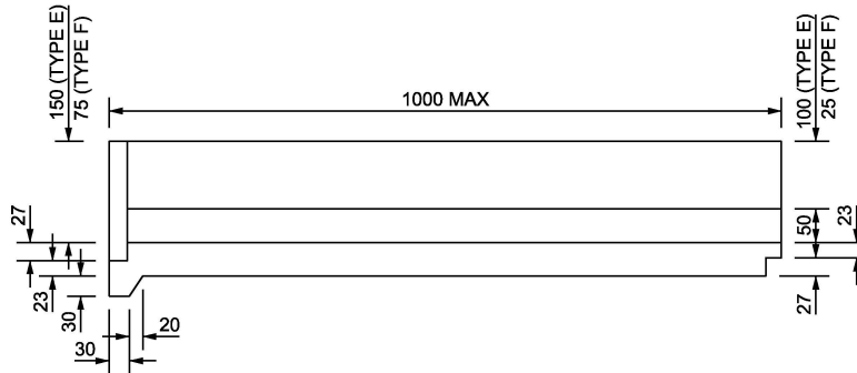
SECTION B
