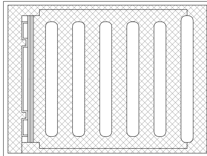
GULLY GRATING DETAIL
