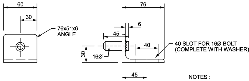
DETAILS OF SWIVEL PIN BRACKET (SECURED TO PLATFORM WITH 16Ø BOLT)
