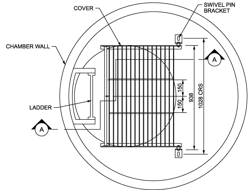
PLAN DETAIL ON GRATING POSITIONED ON LANDING SLAB
