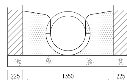
PART SECTION SHOWING BENCHING (FOR PIPES LESS THAN 600Ø)
