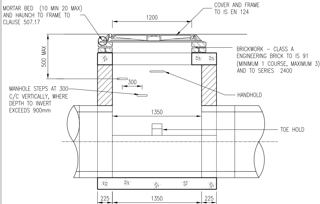
SECTION Y-Y
