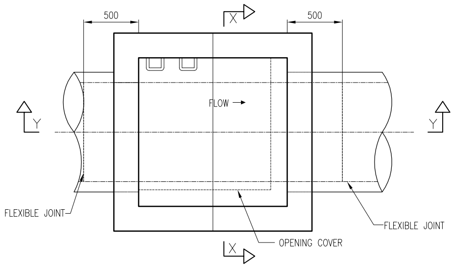
SECTIONAL PLAN
