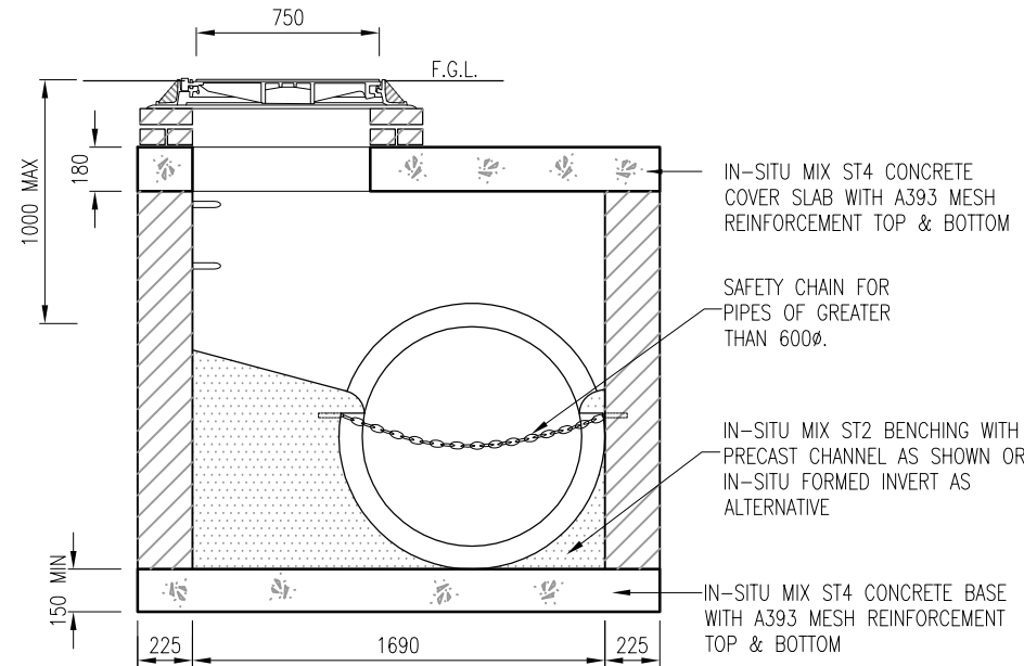
SECTION X-X
