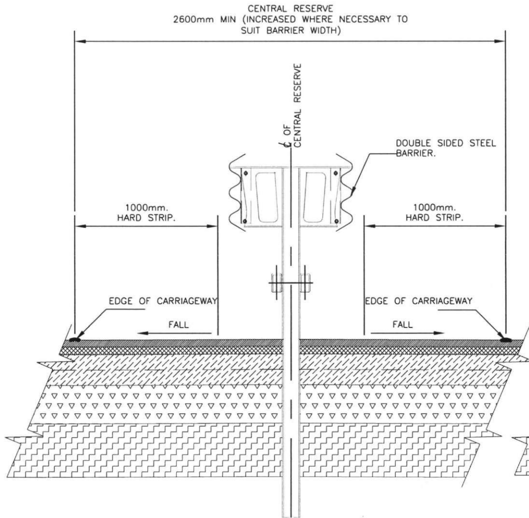
DETAIL WITH NORMAL CROSSFALL
