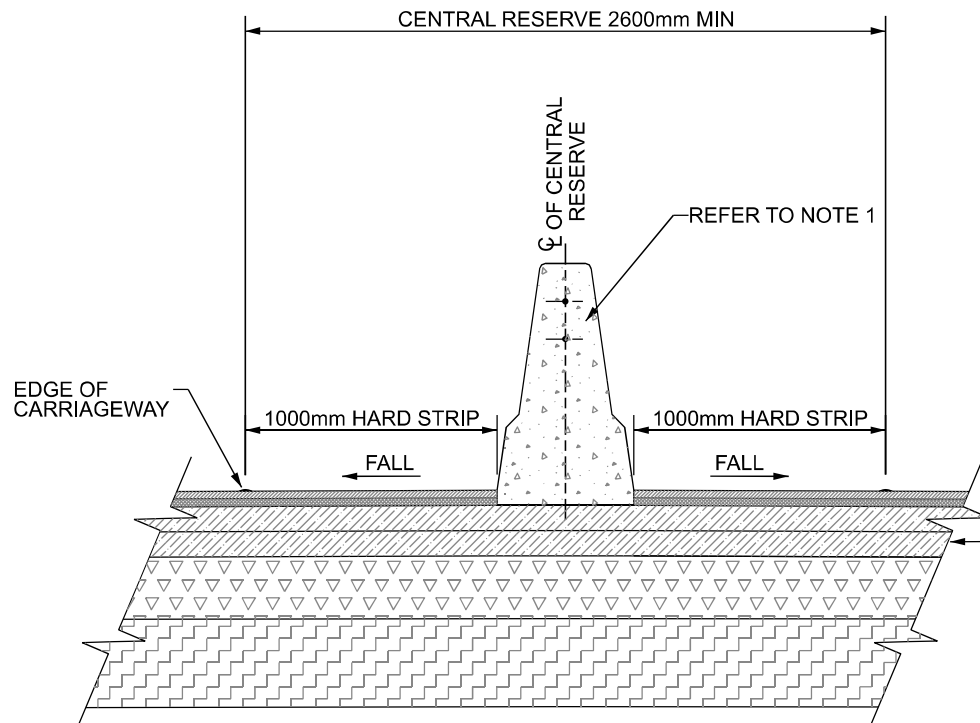
DETAIL WITH NORMAL CROSSFALL
