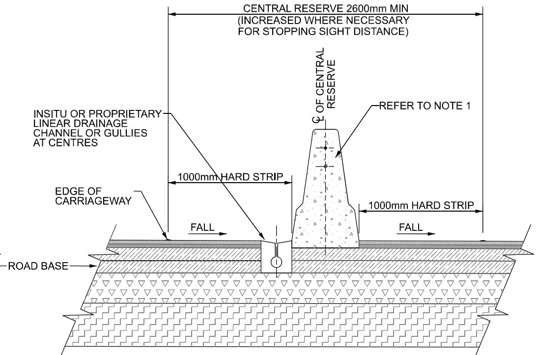
DETAIL WHERE CARRIAGEWAY IS SUPERELEVATED
