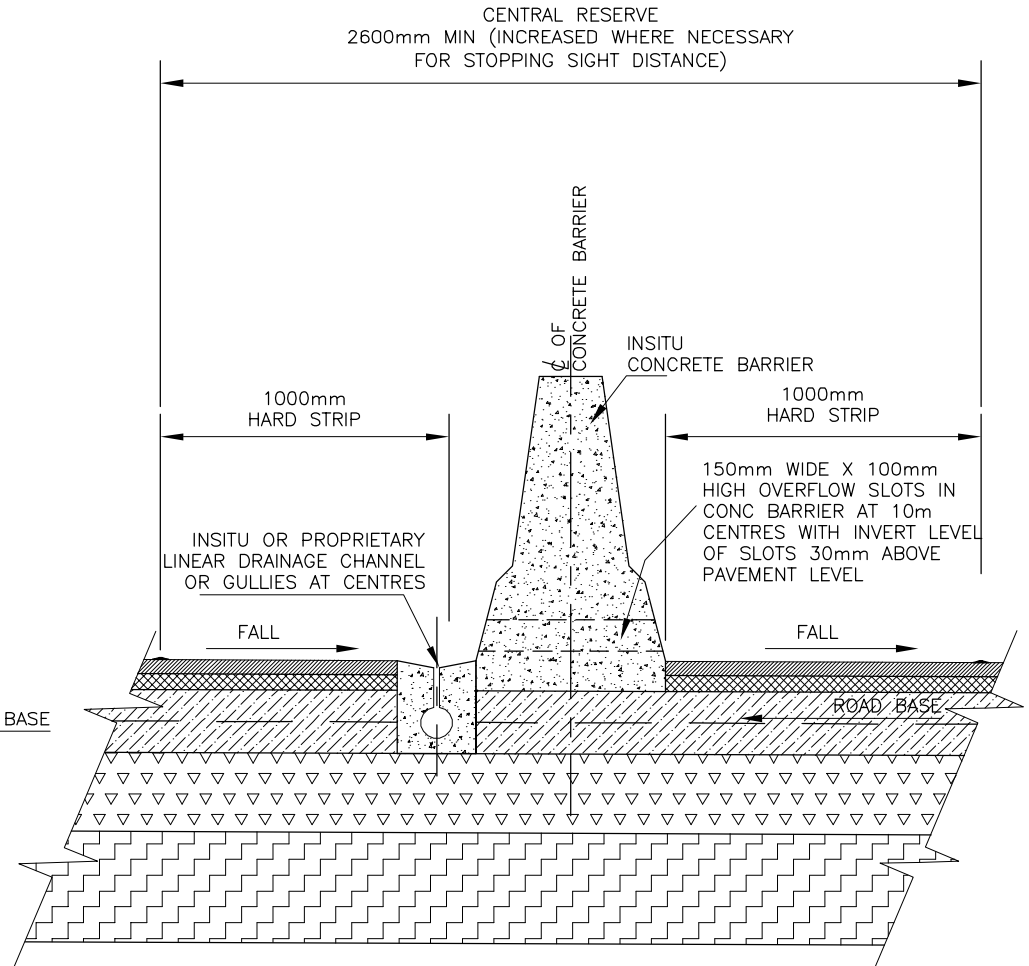
DETAIL WHERE CARRIAGEWAY IS SUPERELEVATED
