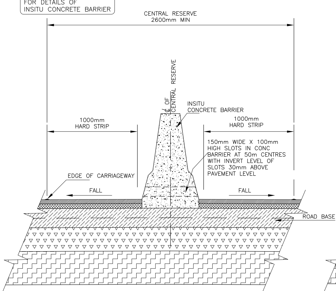
DETAIL WITH NORMAL CROSSFALL
