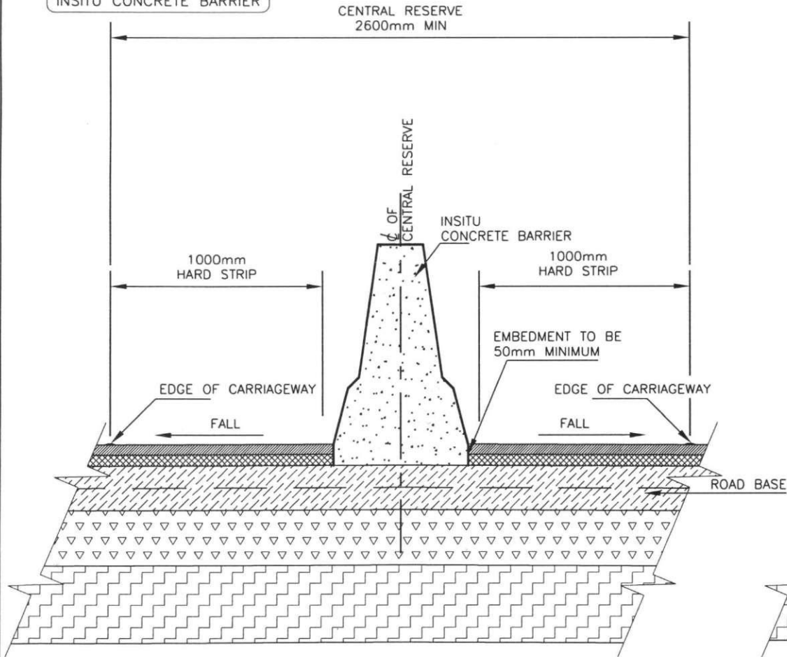
DETAIL WITH NORMAL CROSSFALL
