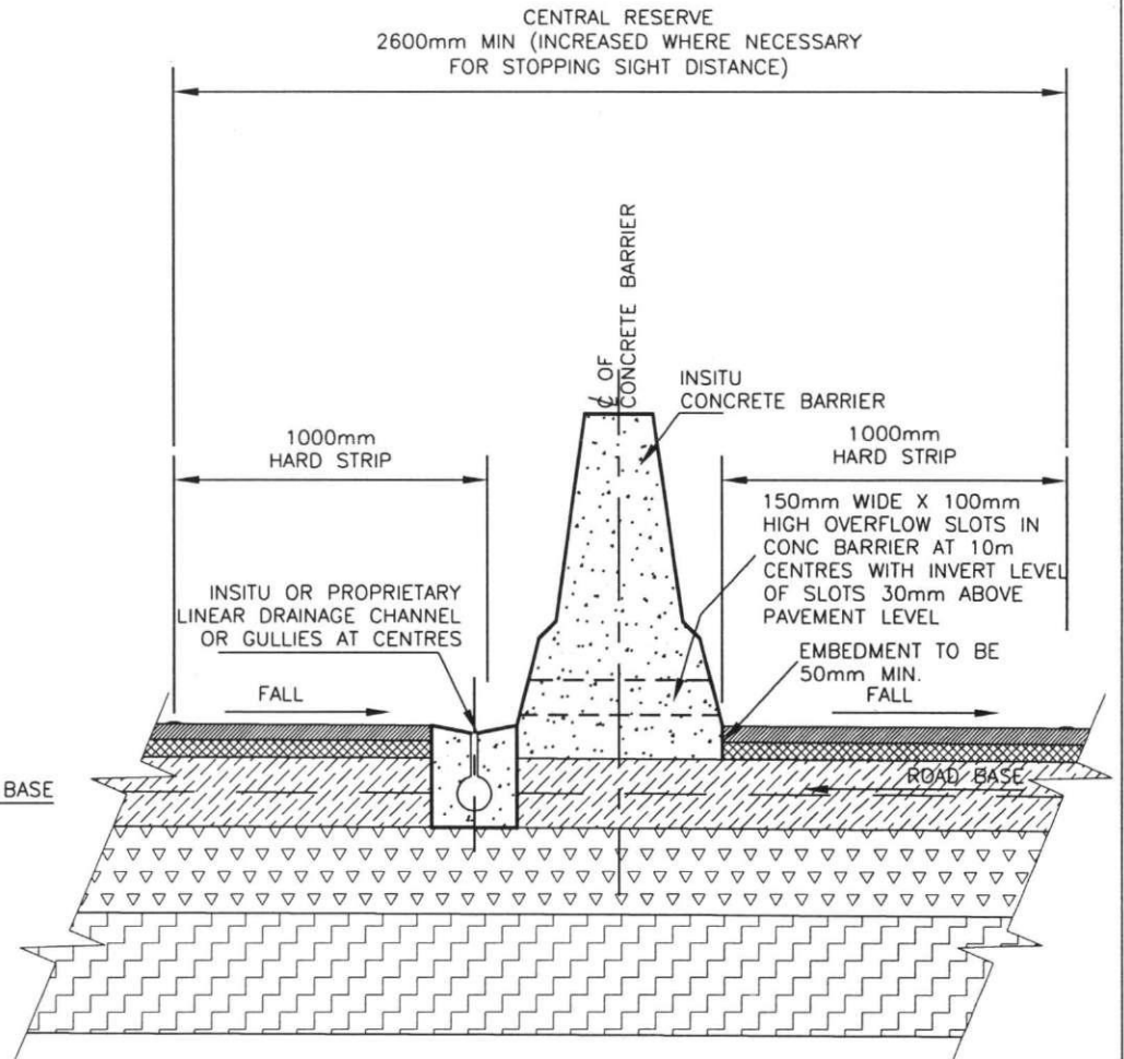
DETAIL WHERE CARRIAGEWAY IS SUPERELEVATED
