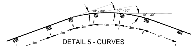
DETAIL 5 - CURVES
