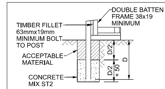
CONCRETE POSTS
