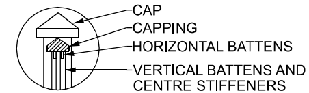
DETAIL A
