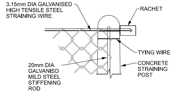
DETAIL SHOWING CHAINLINK STRAINING WIRE ETC.
