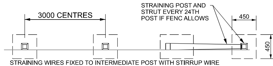
PLAN
