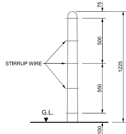
SECTION INTERMEDIATE POST
