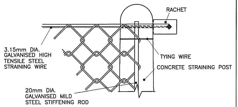
DETAIL SHOWING CHAINLINK STRAINING WIRE ETC
