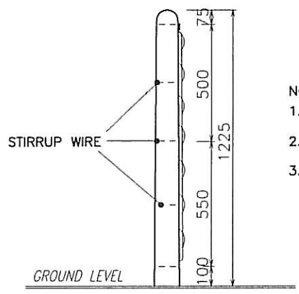
SECTION INTERMEDIATE POST
