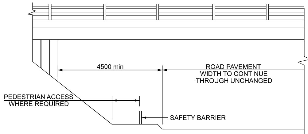
OVERBRIDGE WITH ABUTMENT AT BACK OF VERGE
