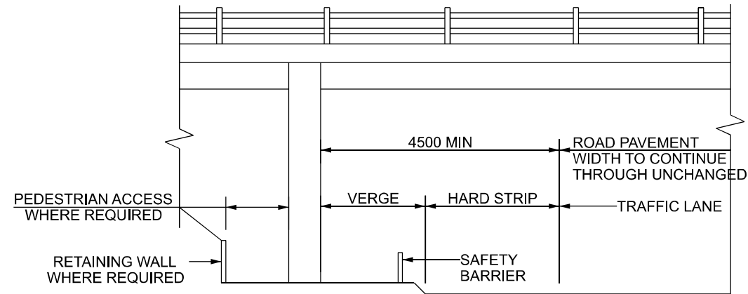
OVERBRIDGE WITH PIER AT BACK OF VERGE
