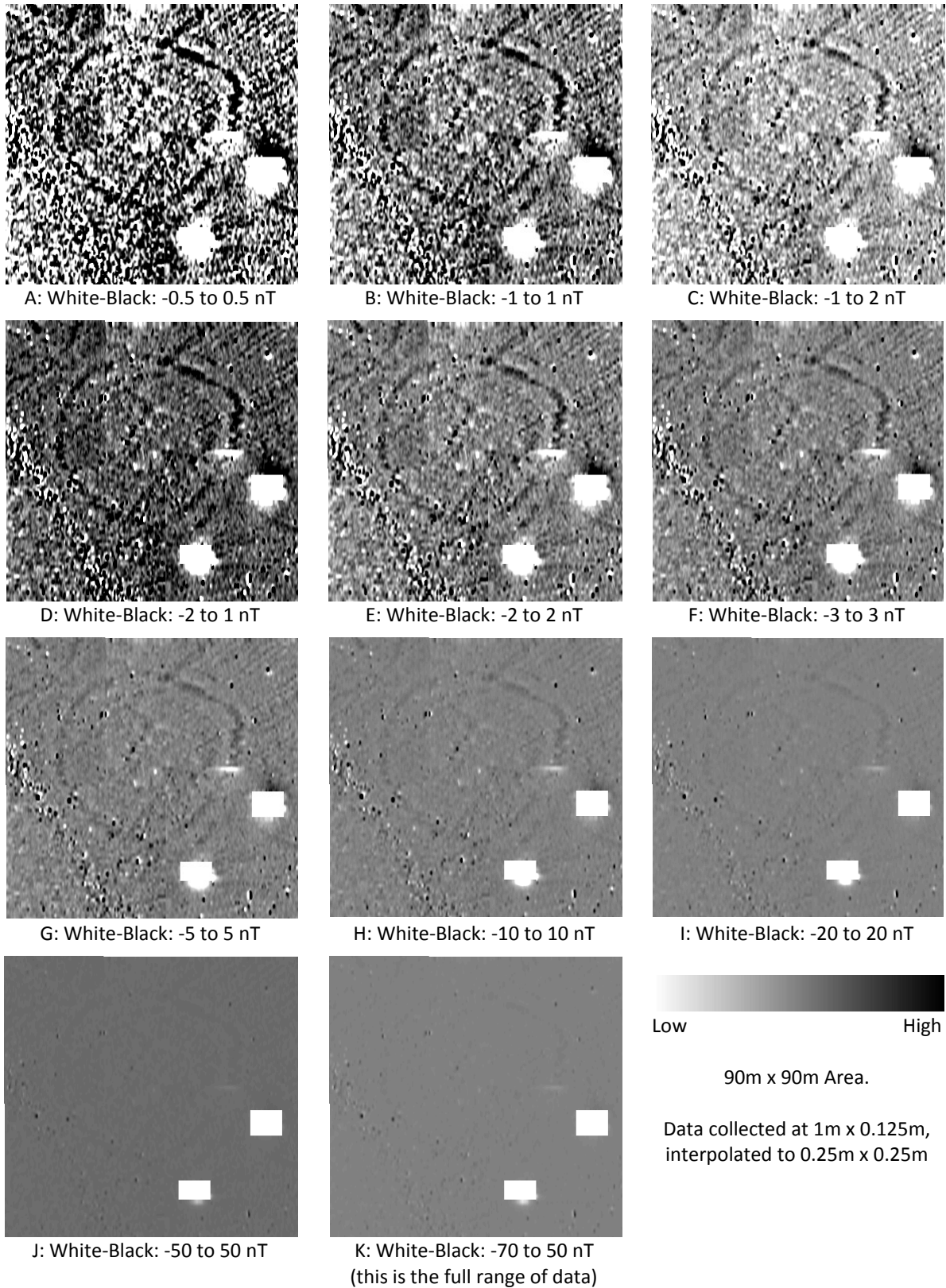
Figure 37. Various clipping ranges for magnetometer data.
