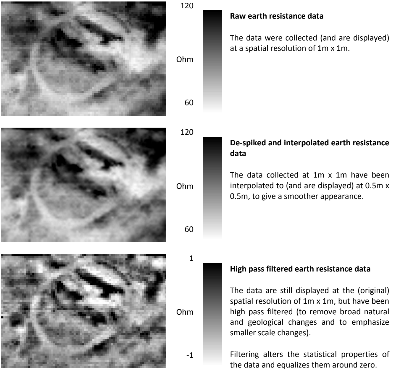
Figure 35. Some common processing steps applied to 2D geophysical data. Data are from Chapelstown enclosure, N9 Carlow Outer Relief Road (GSB 2004)
