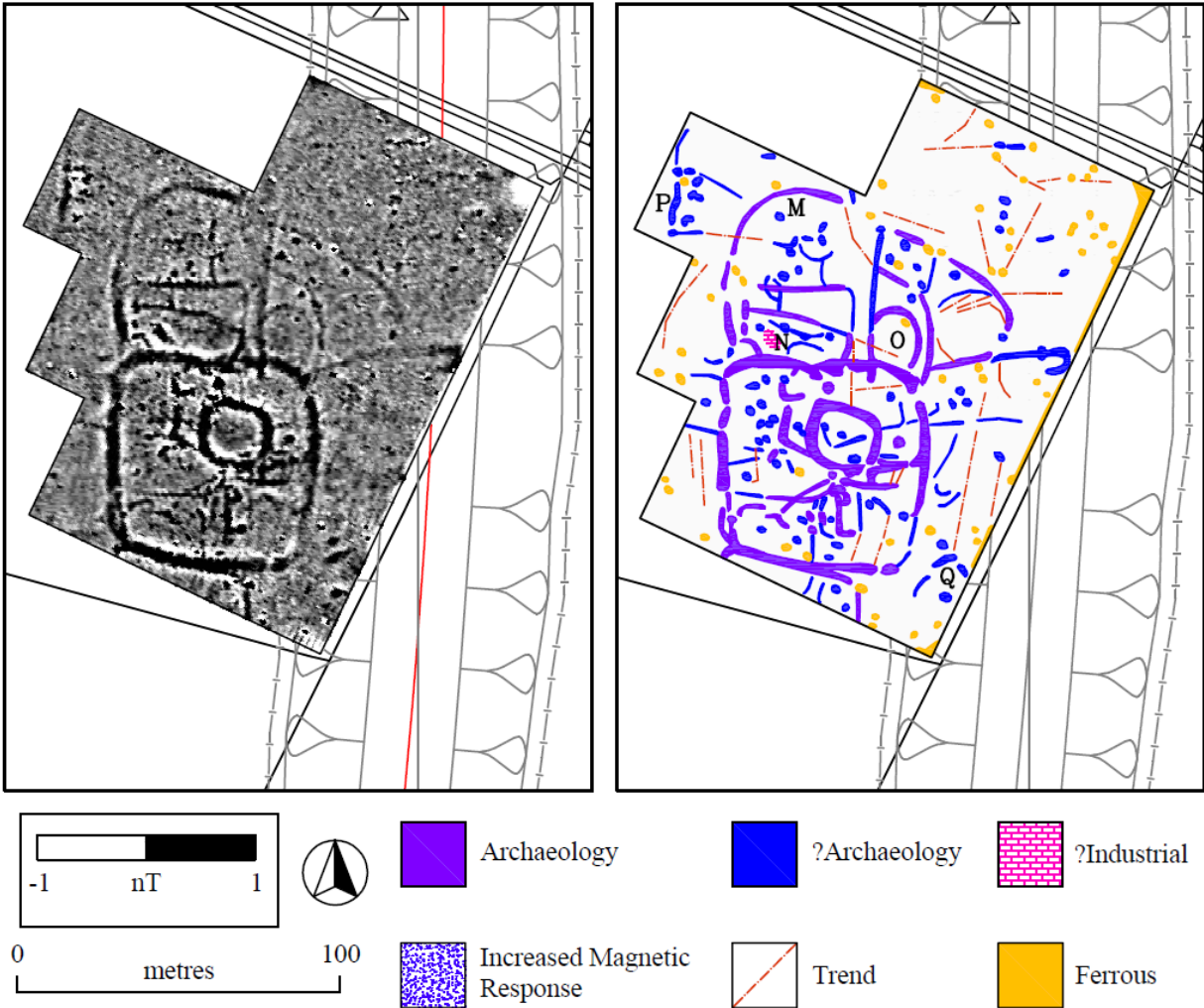
Figure 2. Example of a magnetometer survey.
